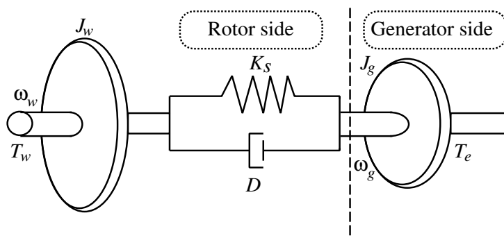
Figure 4. Two-mass shaft model of WECS.
