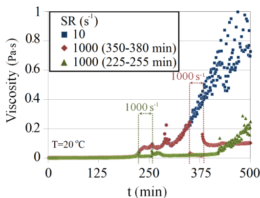
Figure 15. Effect of imposing shear rate ( 1000 \text{ s}^{-1} ) for 30 minutes on 4.5 wt% Na silicate with a pH of 10.35 after 350 min and 225 min of the gelation in comparison to imposing a constant low shear rate ( 10 \text{ s}^{-1} ).
