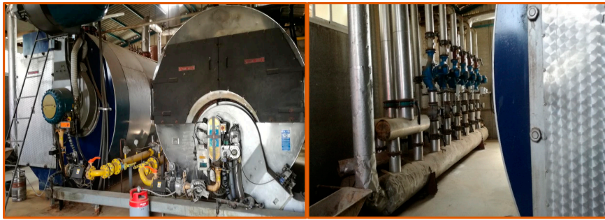
Figure 6. Boilers and water vapor injectors.
