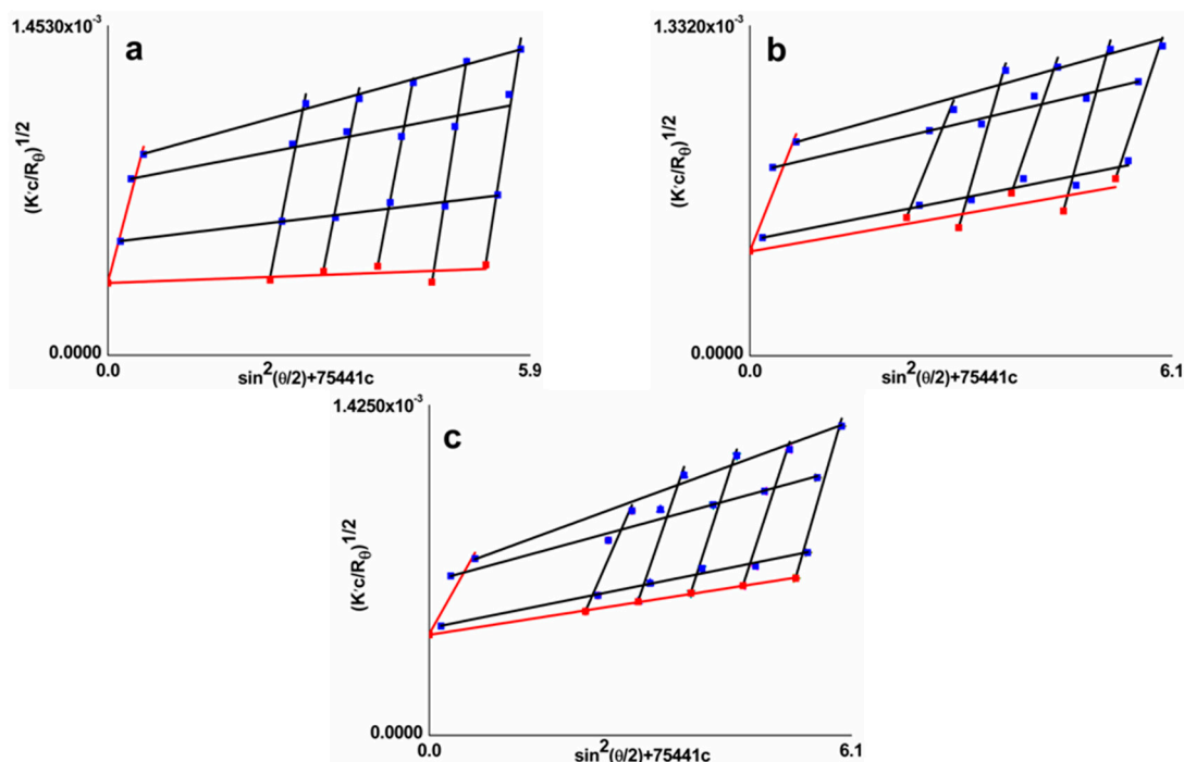
Figure S1. Zimm plot of (a) HPAM; (b) HPMNS-1; (c) HPMNS-2.
