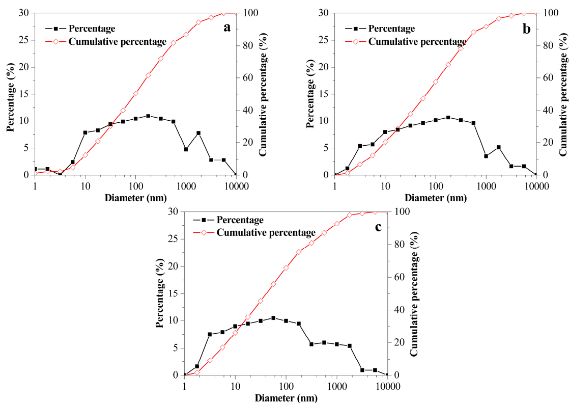
Figure S2. Hydrodynamic radius of (a) HPAM; (b) HPMNS-1; and (c) HPMNS-2.
