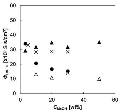
Figure 12. Proton permselectivity ( \phi_{DMFC} ) during DMFC operation at 100 \text{ mA/cm}^2 as a function of methanol concentration in fuel. Sample PEM: solid circles, SF-2; open triangles, SF-5; solid triangles, SF-6; and cross, Nafion112 [31]. Cell temperature, 60 \text{ }^\circ\text{C} .
