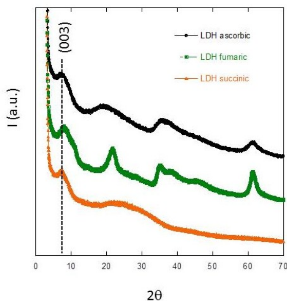
Figure S1. Powder XRD patterns of acids-LDH filler materials.
