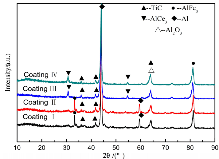
Figure 2. XRD patterns of cladding layer under different laser powers.
