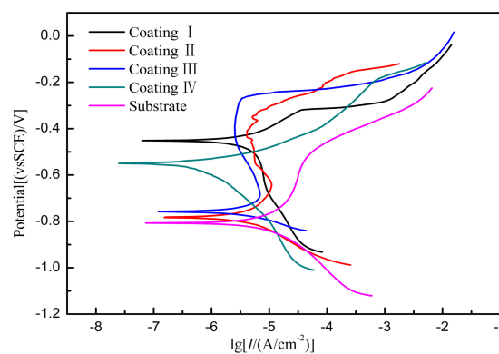
Figure 15. Potentiodynamic polarization of substrate and coatings with different powers.
