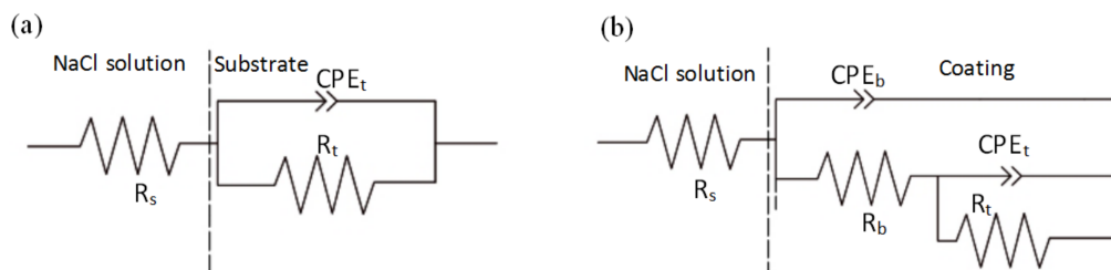
Figure 18. Equivalent circuits of the EIS plots for substrate (a) and coating (b) in the 5% NaCl solution.
