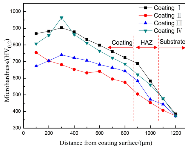
Figure 10. Microhardness profiles of the laser cladding intermetallic composite coatings under different laser power.
