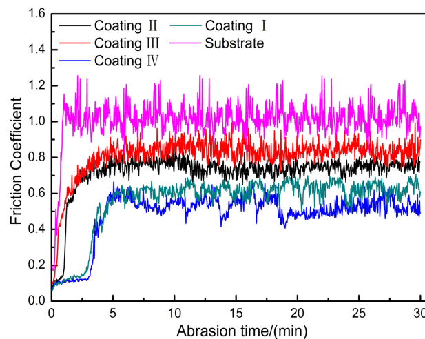
Figure 11. Friction coefficient of cladding layer with time.
