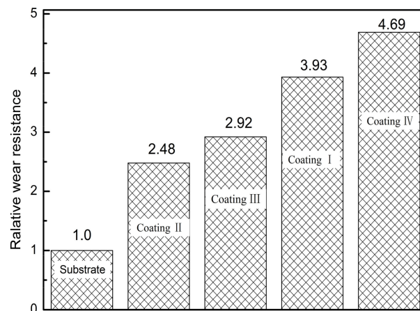
Figure 12. The relative wear resistance of cladding layer.
