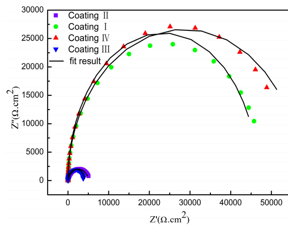
Figure 16. Nyquist of substrate and coatings with different powers.
