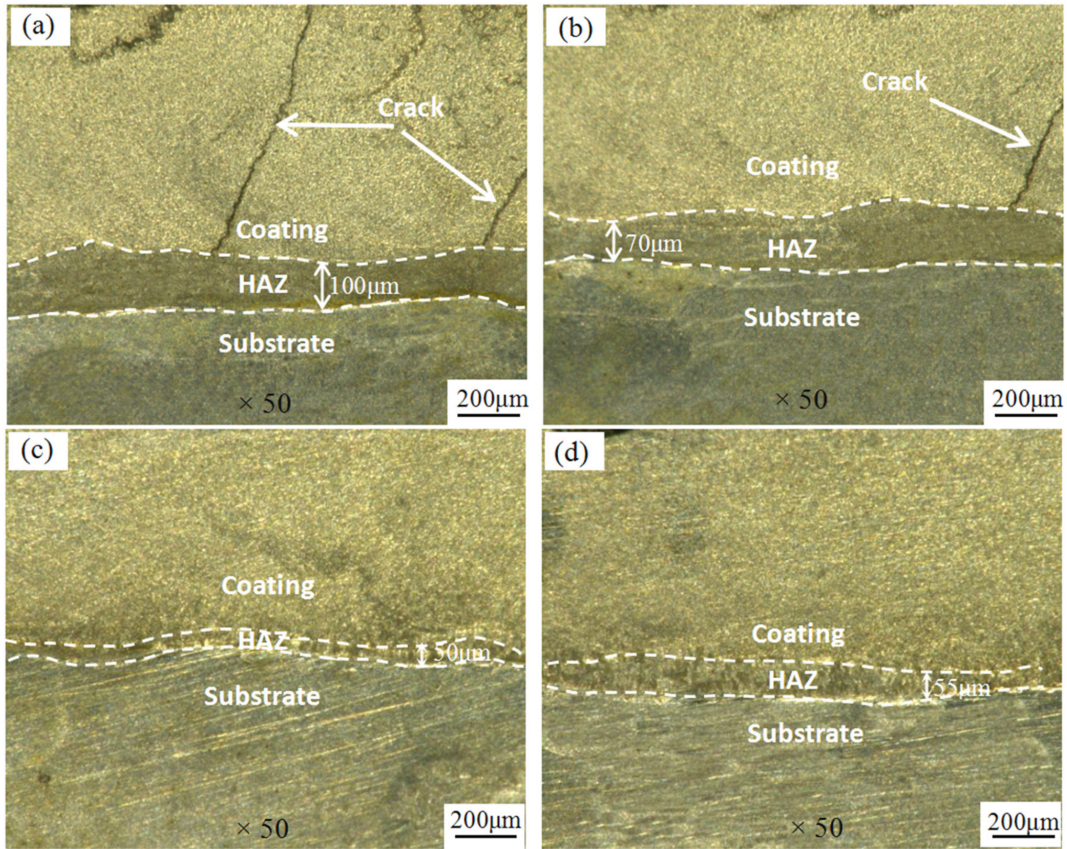
Figure 3. The cross-sectional optical micrographs of coatings, (a) Coating I; (b) Coating II; (c) Coating III; (d) Coating IV.
