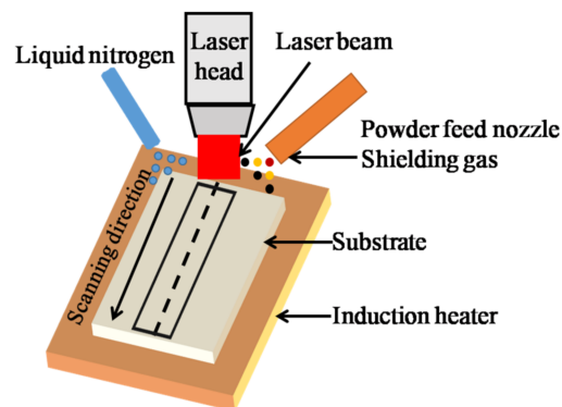
Figure 1. Schematic of laser cladding process.
