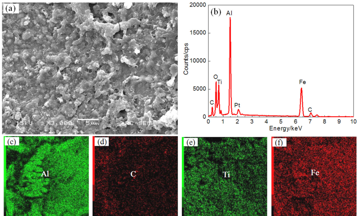
Figure 8. The surface SEM images (a) and EDS analysis result (b) and element content of Plane scan ((c) Al content (d) C content (e) Ti content (f) Fe content) of Coating III.
