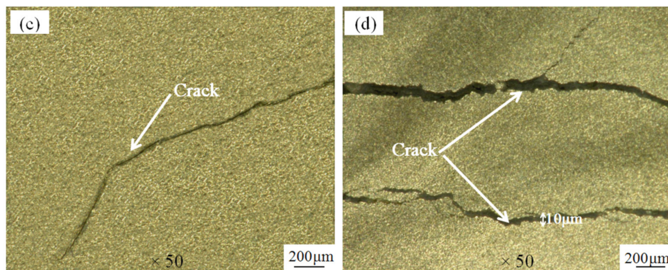
Figure 14. The surface low magnification morphology of the coating: (a) Coating I; (b) Coating II; (c) Coating III; (d) Coating IV.
