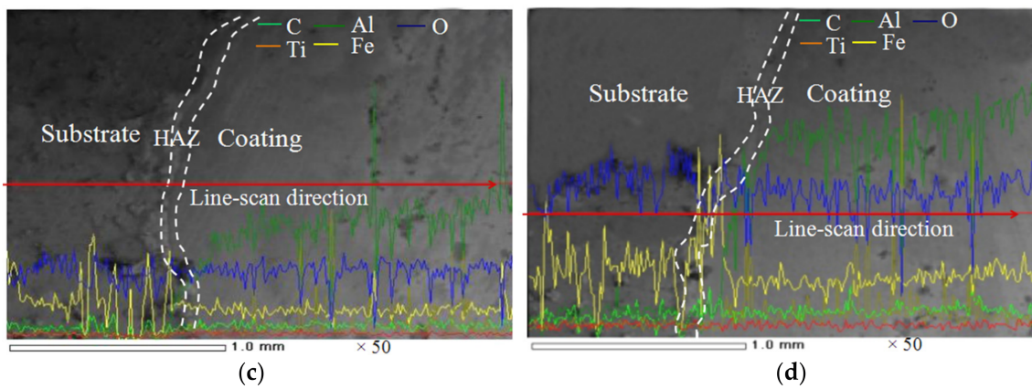
Figure 4. SEM image and EDS line-scan of coating cross-section, (a) Coating I; (b) Coating II; (c) Coating III; (d) Coating IV.
