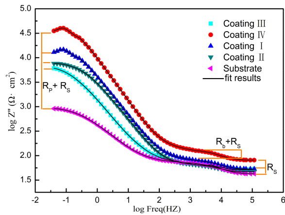
Figure 17. Bode plots of substrate and coatings with different powers.
