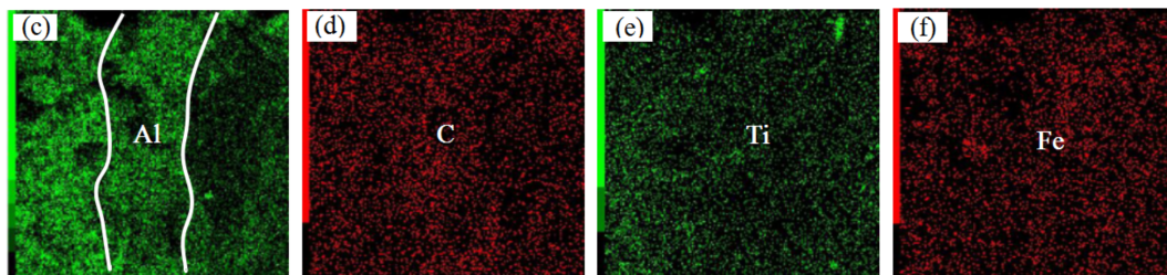
Figure 6. The surface SEM images (a) and EDS analysis result (b) and element content of Plane scan ((c) Al content (d) C content (e) Ti content (f) Fe content) of Coating I.
