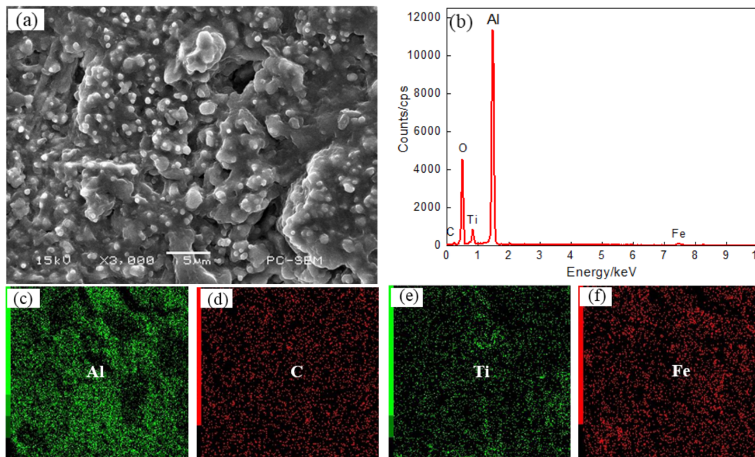
Figure 9. The surface SEM images (a) and EDS analysis result (b) and element content of Plane scan ((c) Al content (d) C content (e) Ti content (f) Fe content) of Coating IV.
