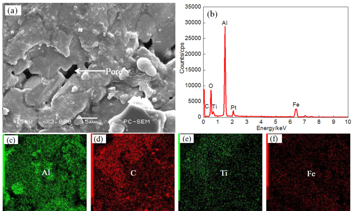
Figure 7. The surface SEM images (a) and EDS analysis result (b) and element content of Plane scan ((c) Al content (d) C content (e) Ti content (f) Fe content ) of Coating II.
