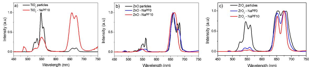
Figure 7. Normalized up-conversion emission spectra of the \text{Er}_2\text{O}_3 -doped \text{TiO}_2 (a), \text{ZnO} (b), and \text{ZrO}_2 (c) particles and of the corresponding particles-containing NaPF0 and NaPF10 glasses with 1.25 wt % of particles.
