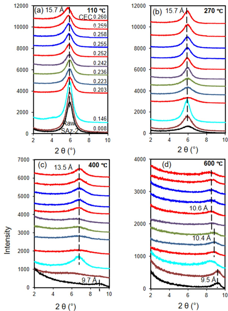
Figure S1. XRD patterns of raw SAz-2 and SAz-2 with different adsorbed amounts without recrystallization from isotherm adsorption for AT under four different heating temperatures (a–d).
