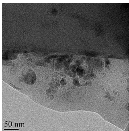
Figure S1. The TEM image of Ag-PDA-RGO.
