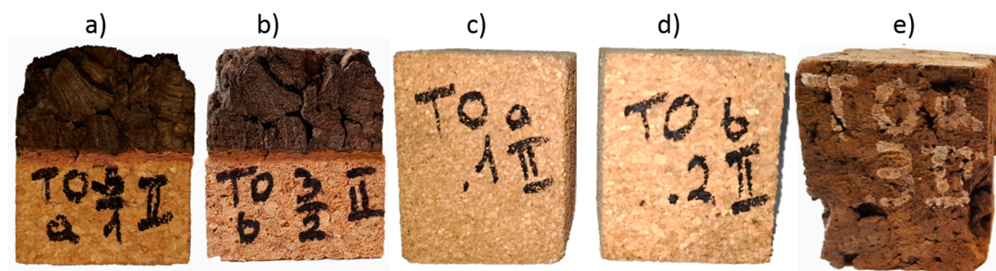
Figure 2. The cork samples after the 100 J impact at 24 °C (a) EC159_AC199A, (b) EC159_AC216, (c) AC199A, (d) AC216, (e) EC159.
