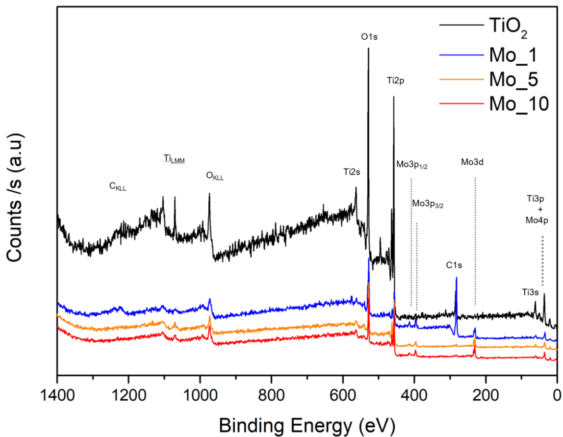
Figure S2. XPS survey spectra of the studied samples [41].
