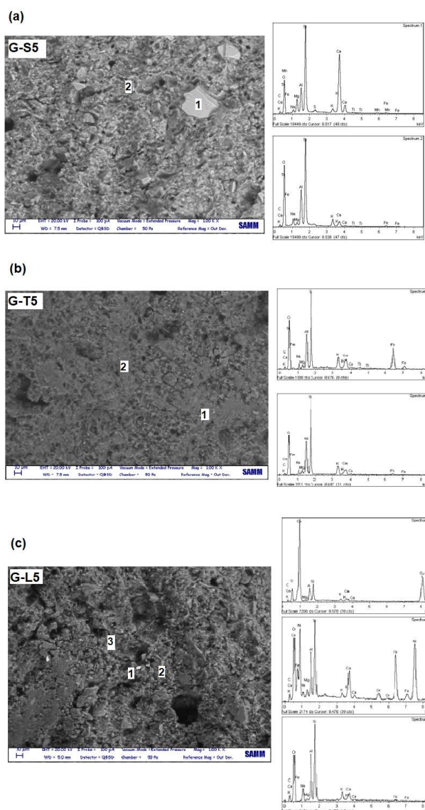
Figure S1. EDS analyses performed on samples containing biomass: (a) G-S5; (b) G-T5; (c) G-L5.
