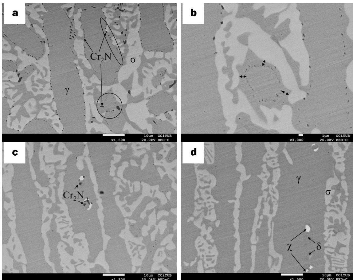
Figure 7. BSE micrographs of SDSS specimen cross-sections after isothermal aging for 10 h at 925 °C. (a) Microstructure of the sample near the surface, indicating austenite ( \gamma ), ferrite ( \delta ), sigma ( \sigma ) and chromium nitrides (dark spots). (b) Higher magnification of a zone near the surface indicating with arrows the displacement of the nitrides from the \gamma/\sigma boundary, forming a circle. (c,d) show the microstructure away from the surface of the sample indicating chi-phase nucleation.
