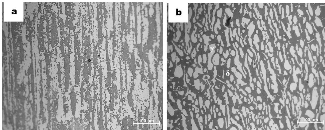
Figure 1. Optical micrographs of DSS (a) and SDSS (b), after annealing process at 1080 °C for 30 min. Homogenous microstructure of relatively equal distribution of austenite and ferrite phases is shown after being etched by modified Murakami chemical reagent [22].
