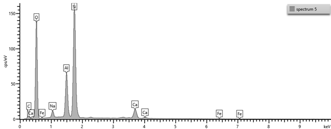
Figure S3. EDX spectra obtained from single spot analyses (areas are marked in Figure 4, third panel).
