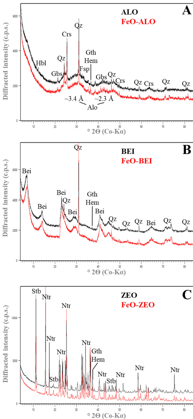
Figure S1. XRD patterns of adsorbents collected after the Ba adsorption.
