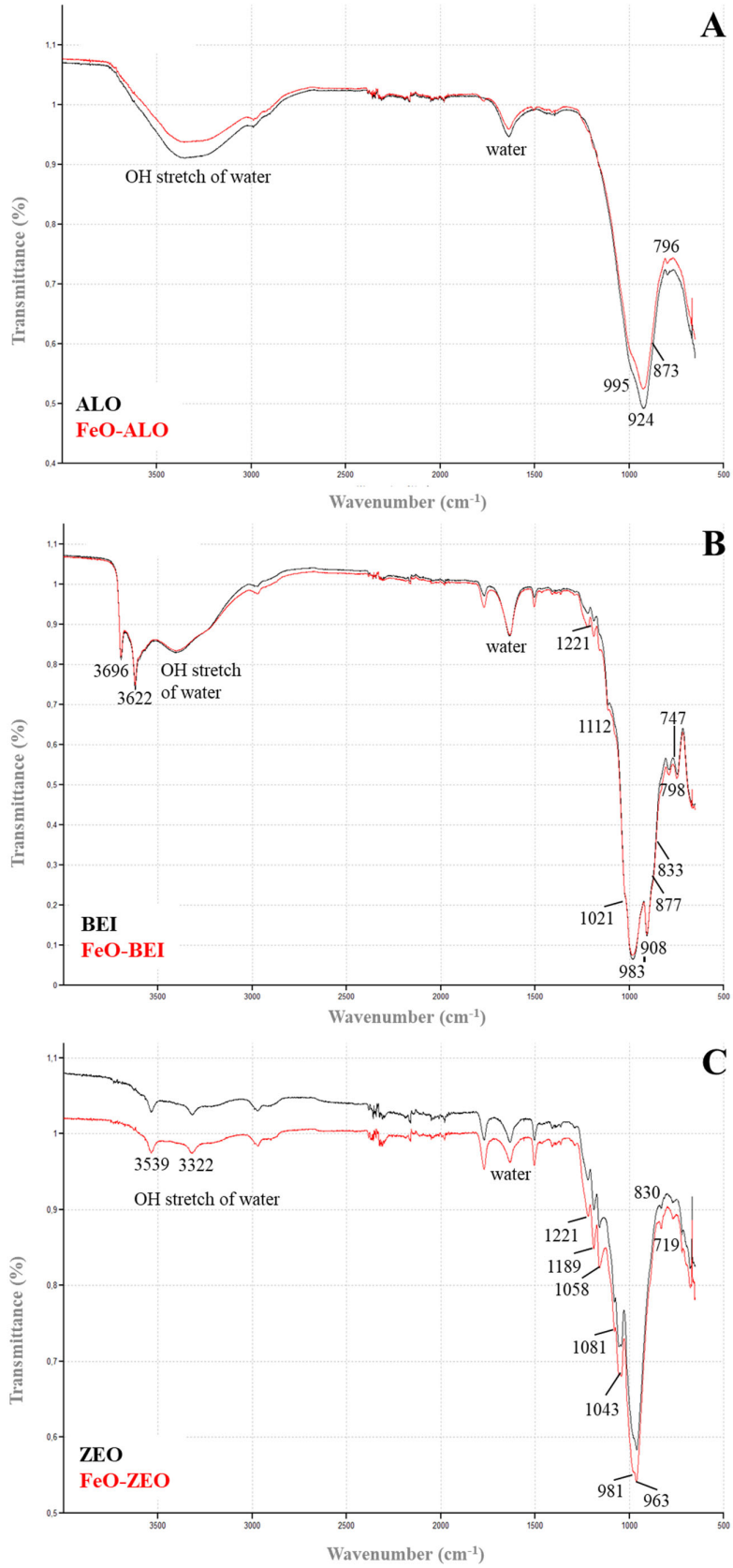
Figure S2. FTIR spectra of adsorbents collected after the Ba adsorption.
