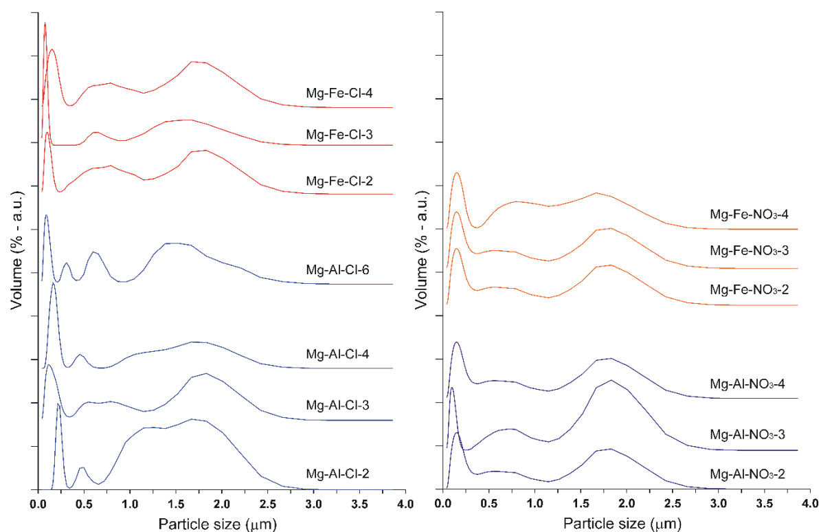
Figure S1. Particle size distribution of the raw LDH samples (y axis—Volume (% a.u.)—one spacing on the y axis corresponds to 4%).
