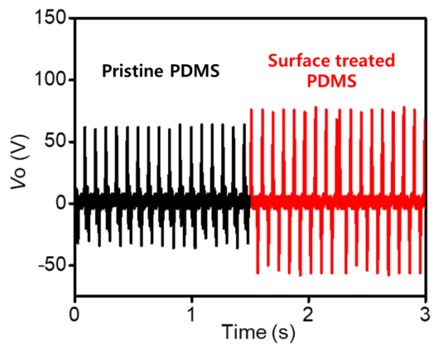
Figure S1. Output voltages generated from the TENG with the pristine PDMS contact layer and the ozone treated PDMS contact layer.
