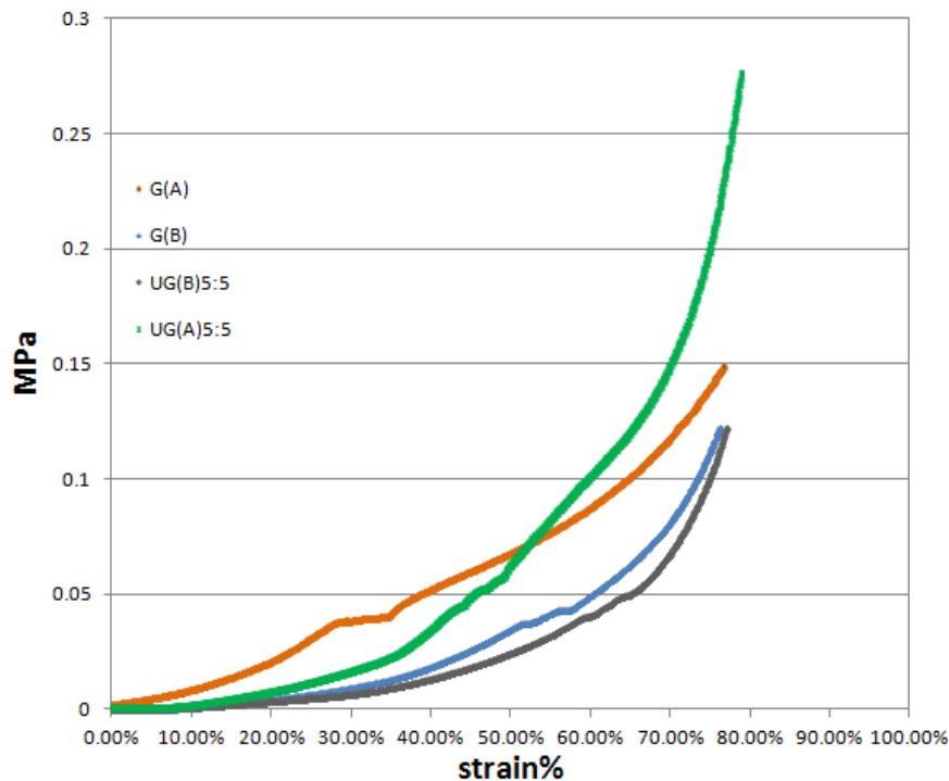
Figure S1. Representative stress-strain curves of UG scaffolds.
