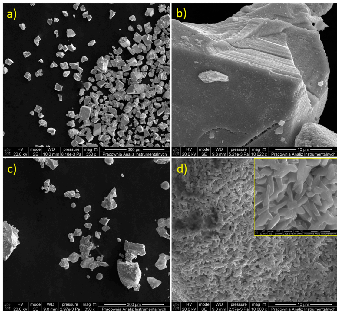
Figure 2. SEM images of (a,b) bulk and (c,d) hydrated and non-crystalline \text{WO}_3 .
