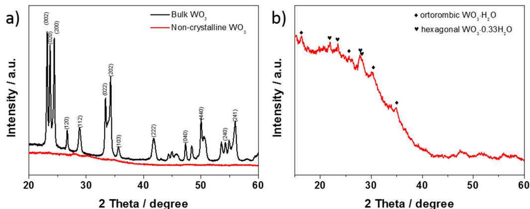
Figure 5. XRD patterns of (a) bulk and hydrated and non-crystalline \text{WO}_3 , (b) only hydrated and non-crystalline \text{WO}_3 .
