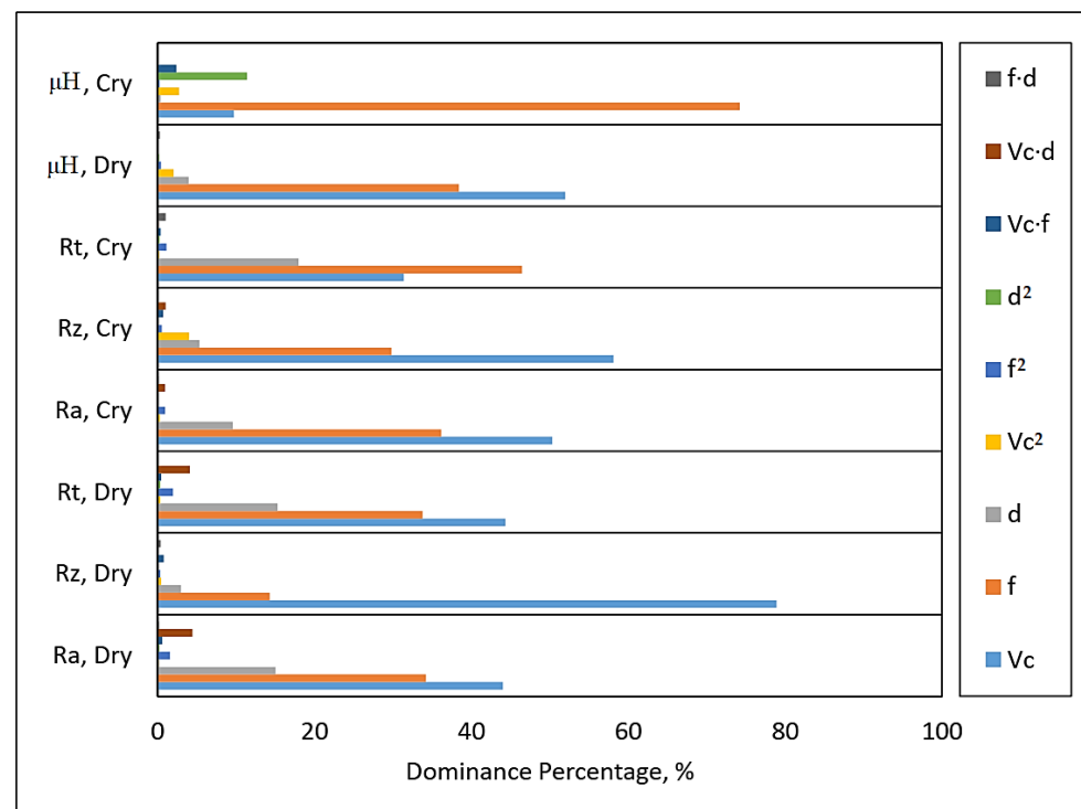
Figure 5. Dominance percentage of each process parameter in different turning conditions.
