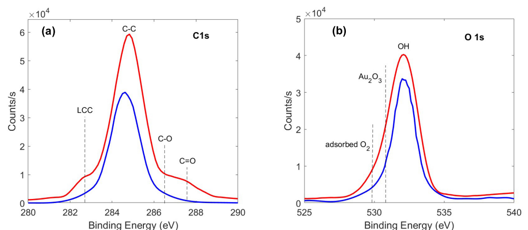
Figure 6. C 1s (a) and O 1s (b) XPS profiles of Au (blue line) and Au@LCCs (red line) nanosystems.
