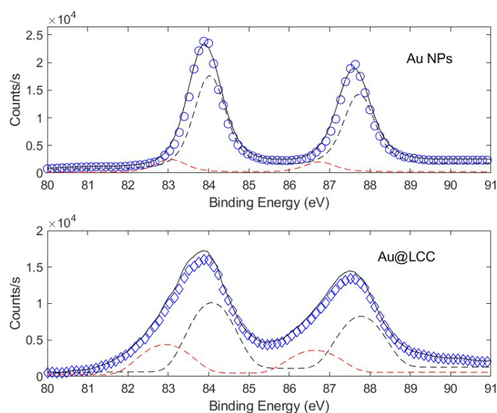
Figure 7. Au 4f lineshape deconvolution for NPs ( top ) and AuNPs@LCC ( bottom ) samples.
