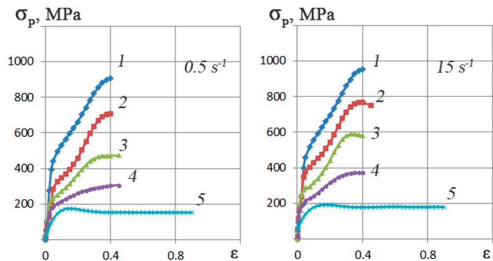
Figure 4. The Zr-2.5%Nb alloy by the Gleeble 3800 plastometer flow curves for the compression method in the strain rate range of 0.5 – 15 \text{ s}^{-1} at temperatures: 1– 20^\circ\text{C} ; 2– 200^\circ\text{C} ; 3– 350^\circ\text{C} ; 4– 500^\circ\text{C} ; 5– 770^\circ\text{C} .
