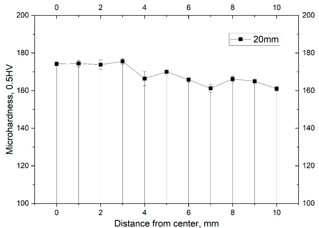
Figure 12. The results of the study of microhardness HV 0.5 from the periphery to the center of the Zr-2.5%Nb alloy bar after rolling on the RSP-14/40 rolling mill.
