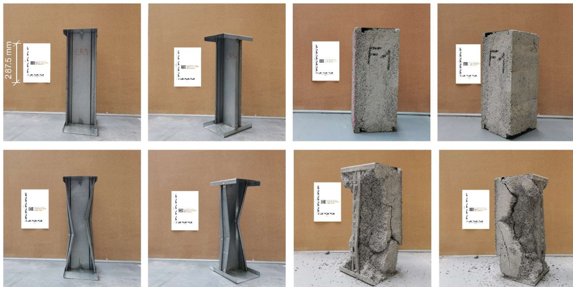
Figure 8. Comparison of test specimens for the composite system. On the left: plain steel profiles connected to horizontal U-profiles at the top and bottom by spot welding. On the right: identical steel profiles embedded in the LAC+. Compression tests for sheet steel profiles ( left ) versus composite specimens ( right ) before ( top ) and after ( bottom ) the test.
