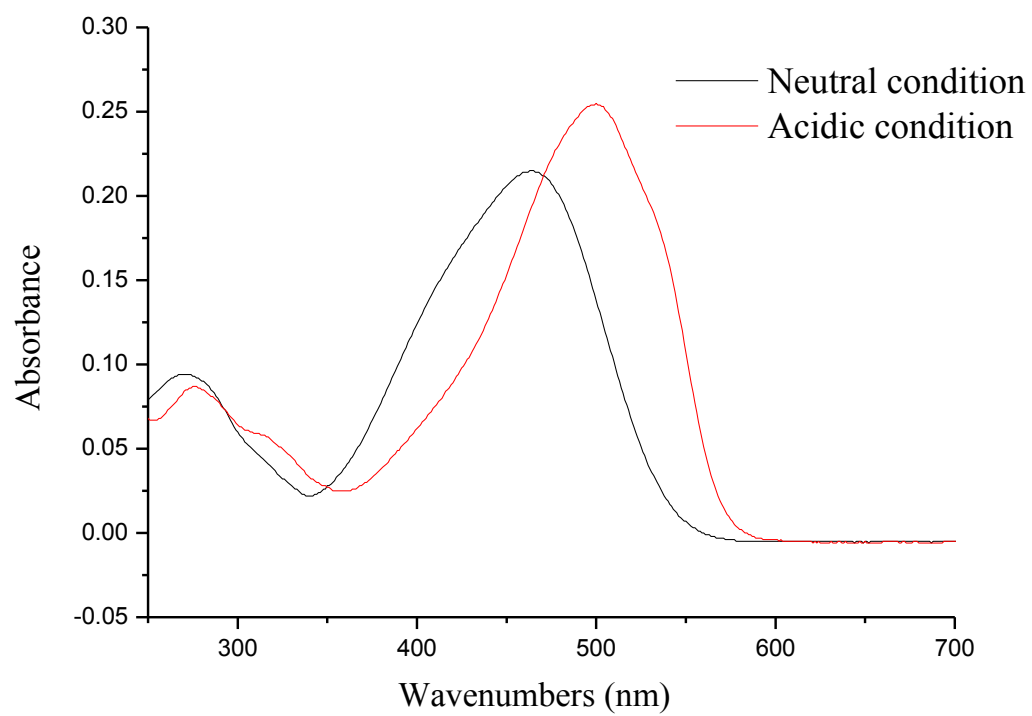
Figure S1. UV-vis spectra of methyl orange under neutral condition and acidic condition.
