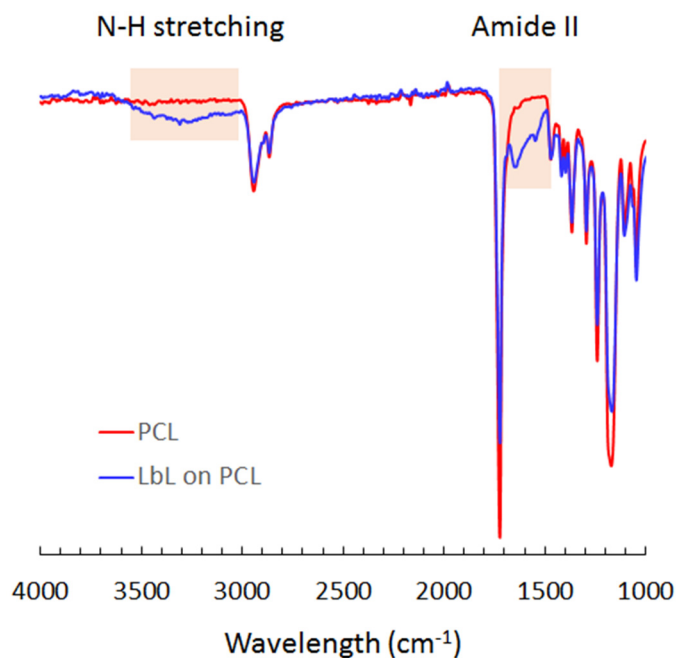
Figure S1. FTIR spectrum of bare PCL nanofibers and LbL coated PCL nanofibers were measured for confirming the existence of LbL multilayer on PCL nanofibers, respectively.
