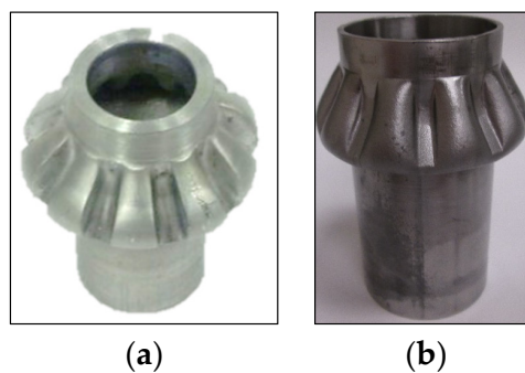
Figure 16. Bevel gear: AL6061(a) and SS304 (b).
