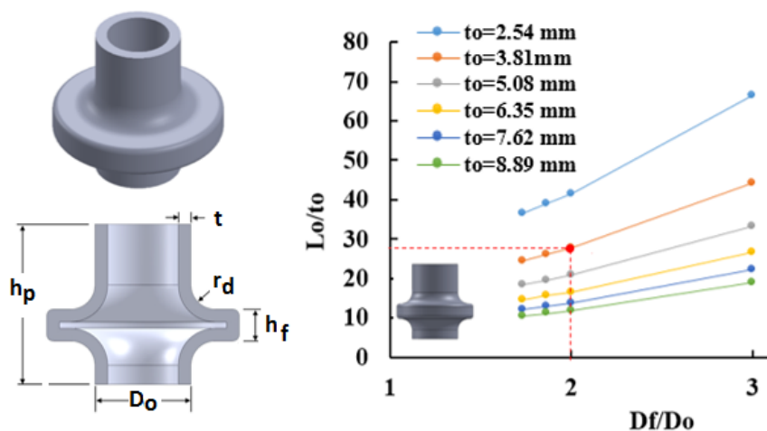
Figure 4. Process window for hollow vessel with flange height h_f = 12.7 mm.
