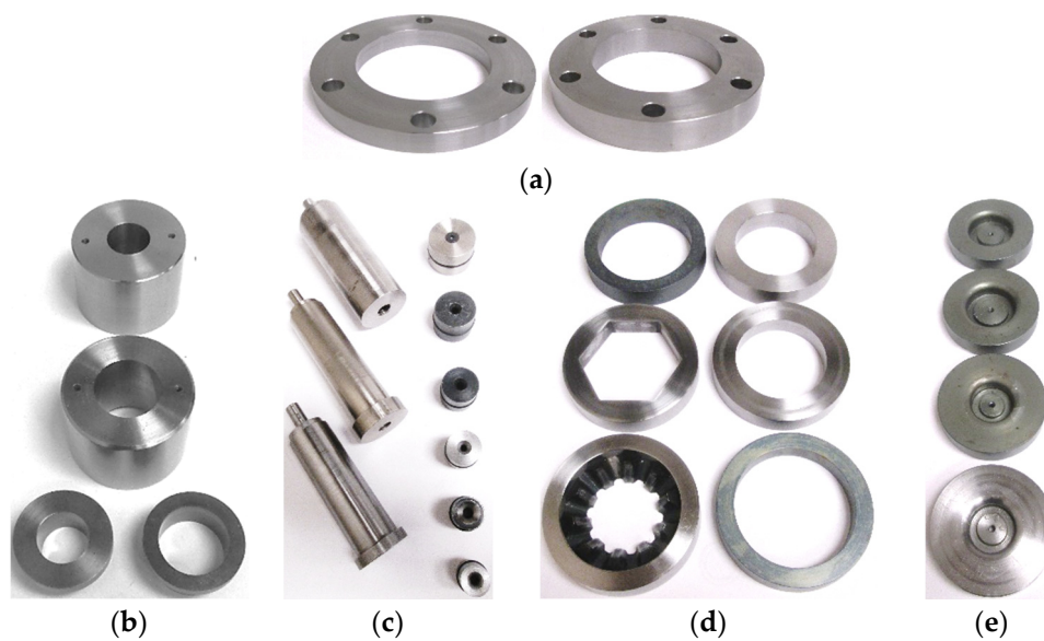
Figure 11. Experimental setup parts: (a) Support rings; (b) guiding zone inserts; (c) punch assemblies; (d) die inserts; and (e) bottom sealing inserts.
