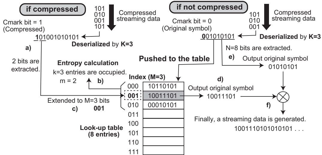
Figure 3. Decompression mechanism in ASE coding. The decompressor checks the first bit of the compressed data stream. As shown in the left side, (a) when the Cmark is set, (b) the entropy calculation generates two due to the occupation of the look-up table. From the data stream, two bits are picked up as a compressed data. Subsequently, (c) the data are extended to three bits. (d) It is used as an index of the look-up table and outputs the data in the associated table entry as the original symbol. Besides, (e) when the Cmark is reset, the original symbol is received. Eight bits are picked up from the stream and it is generated as the original symbol. Concurrently, the symbol is registered to the table.
