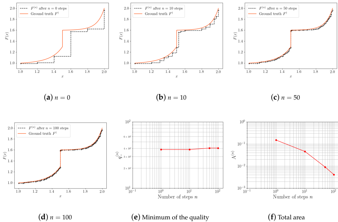
Figure 5. Evolution of F^{(n)} and the minimum of the quality and the total area as functions of the iteration count, n , for a discontinuous ground truth F^\dagger with \varepsilon = 10^{-4} .
