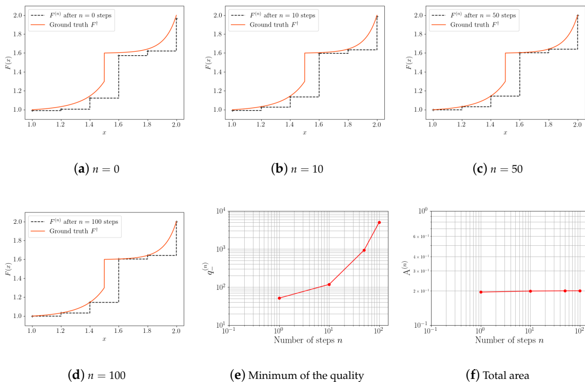
Figure 6. Evolution of F^{(n)} and the minimum of the quality and the total area as functions of the iteration count, n , for a discontinuous ground truth F^\dagger with \varepsilon = 10^4 .
