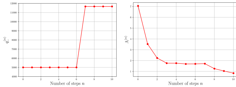
(a) Evolution of the minimum of the quality. (b) Evolution of the total area.
