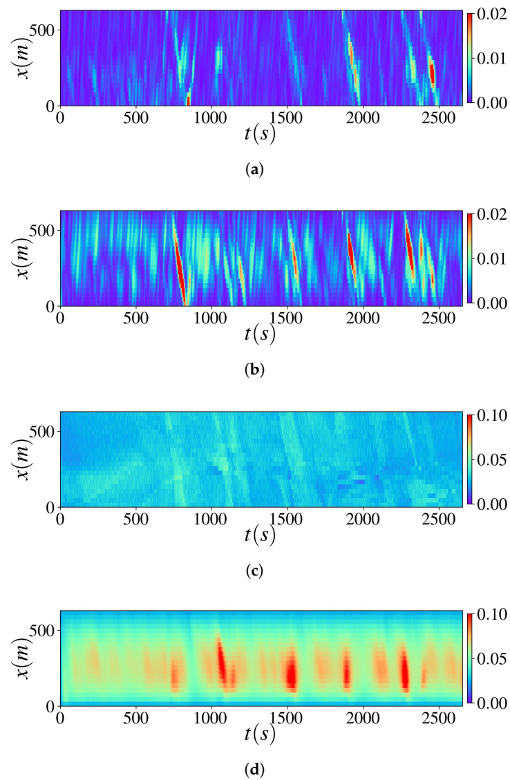
Figure A2. Error heatmaps of the EKF and TrafficFlowGAN. (a) SE_\rho(x,t) of the TrafficFlowGAN; (b) SE_\rho(x,t) of the EKF; (c) prediction’s standard deviation of the traffic density of the TrafficFlowGAN; (d) prediction’s standard deviation of the traffic density of the EKF.
