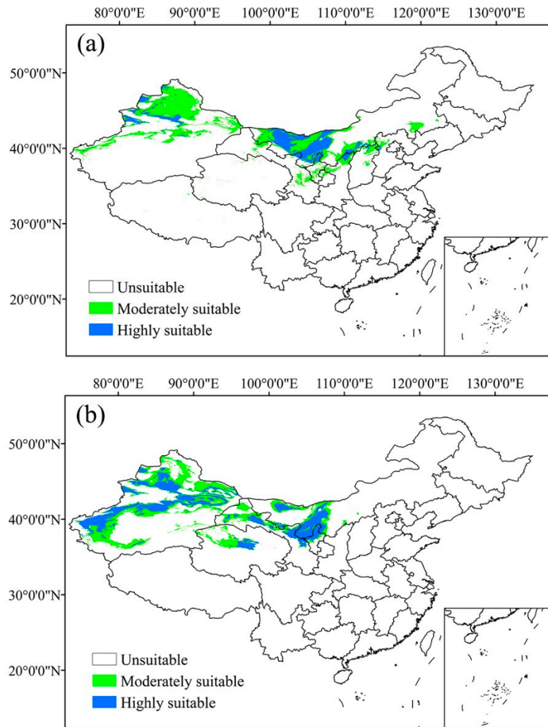
Figure S1: Potential comprehensive habitat suitability of C. deserticola (a) and H. ammodendron (b) in current.
