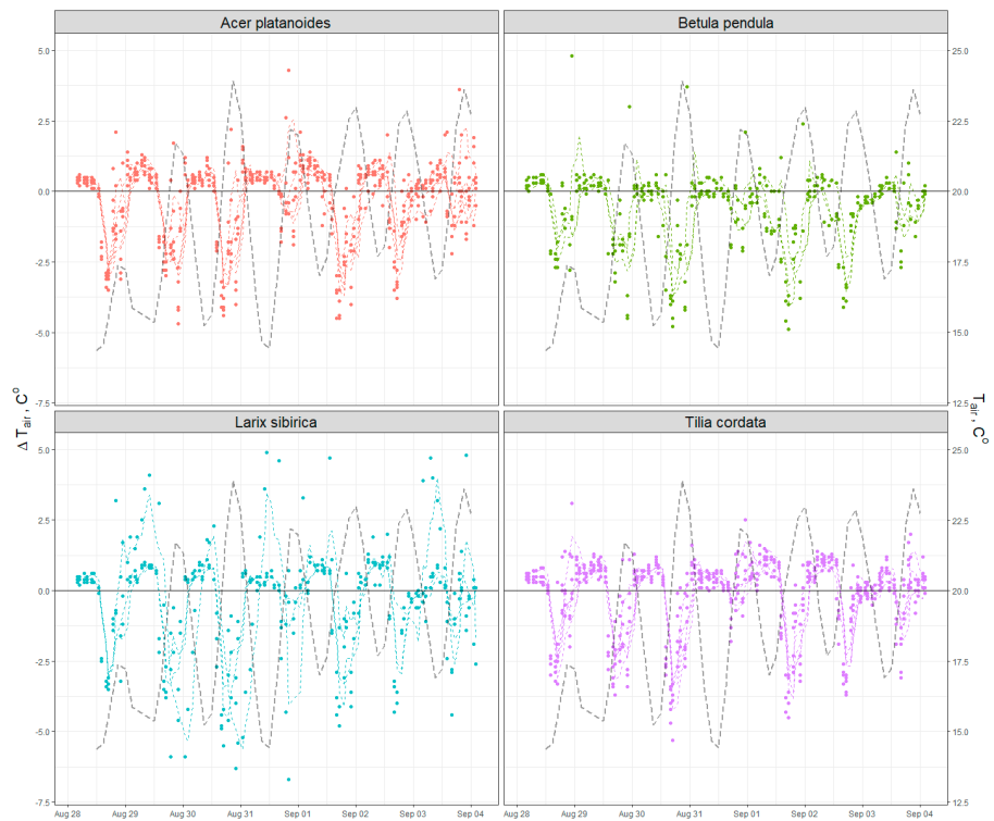
Figure A1. Daily dynamics example of the air temperature ( T_{air} —dashed line) and the difference ( \Delta T_{air} —colored line) under and outside of the canopy ( T_{air} — T_{T_{air}} ).
