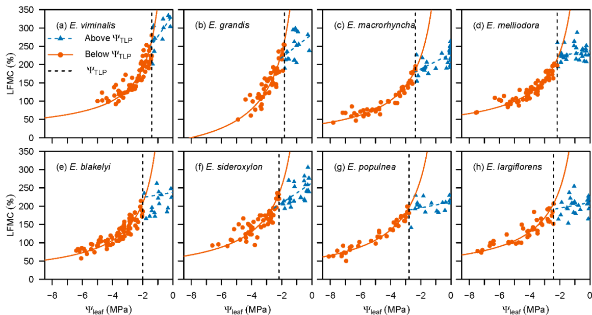
Figure 3. Decline in LFM and \Psi_{leaf} modelled using Equation (3) (for data > \Psi_{TLP} ) and Equation (4) (for data < \Psi_{TLP} : -1/\Psi_{leaf} versus LFM), for saplings of eight Eucalyptus species. Species are ordered by increasing moisture index (ratio of precipitation to potential evapotranspiration) from climate of origin, i.e., E. largiflorens is from the most arid climate. Regressions for all species were statistically significant ( p < 0.05 ), except the slope of the linear regression above the \Psi_{TLP} for the following species: E. grandis , E. melliodora , E. blakelyi , E. populnea and E. largiflorens . (a) E. viminalis ; (b) E. grandis ; (c) E. macrorhyncha ; (d) E. melliodora ; (e) E. blakelyi ; (f) E. sideroxylon ; (g) E. populnea ; (h) E. largiflorens .
