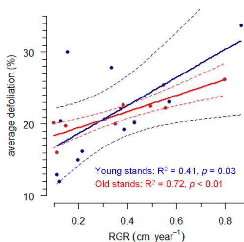
Figure 6. Lineal regression between the relative growth rate (RGR, calculated for the period 2001–2007) and average defoliation in 2017 of young (blue lines and symbols) and old (red lines and symbols) Abies pinsapo trees. The dashed lines show the 95% prediction intervals.
