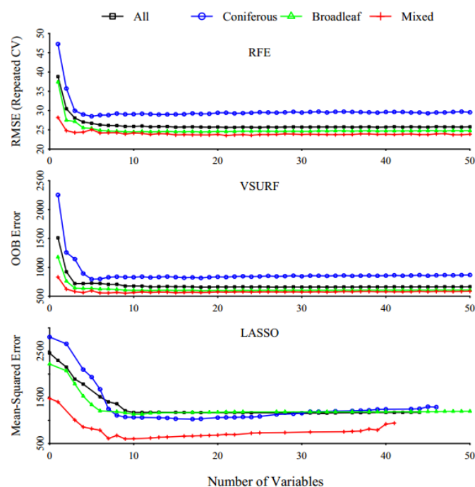
Figure 3. The changes in the accuracy of three feature selections (recursive feature elimination (RFE), least absolute shrinkage and selection operator (LASSO), variable selection using random forests (VSURF)) with the number of variables. Each curve represents an independent model, and different colors indicate different forest types.
