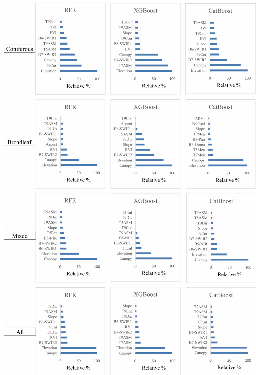
Figure A1. Variable importance ranking for the different forest types by combining feature selection method (LASSO) and three machine learning algorithms (RFR, XGBoost, and CatBoost).
