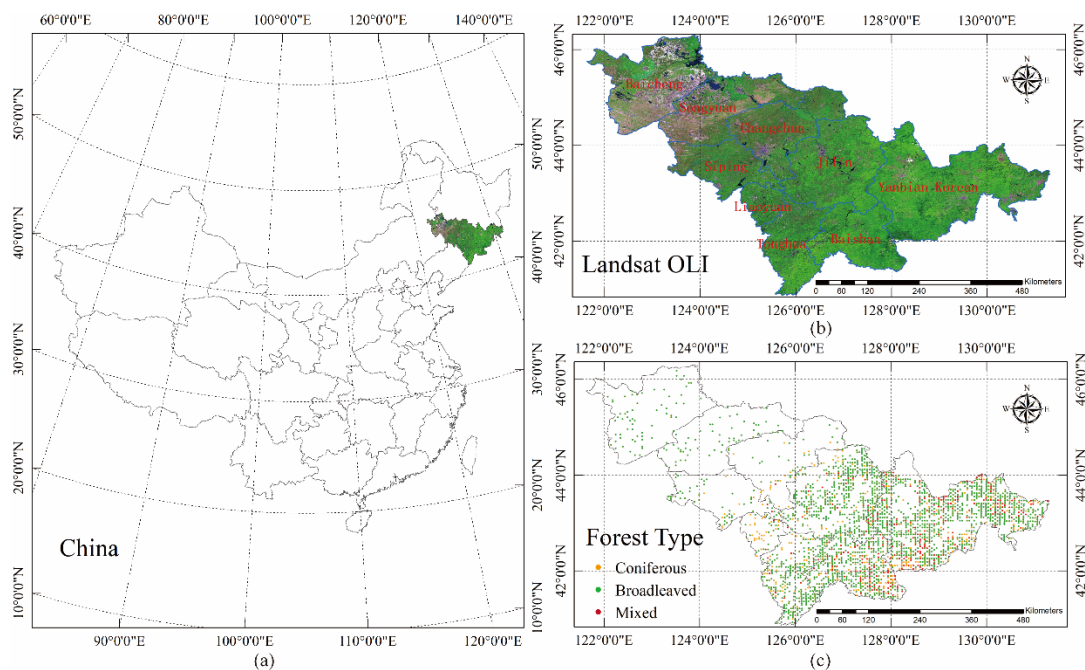
Figure 2. (a) Study area in Jinlin Province, China; (b) false color image of Landsat OLI; and (c) the distribution of forest types.
