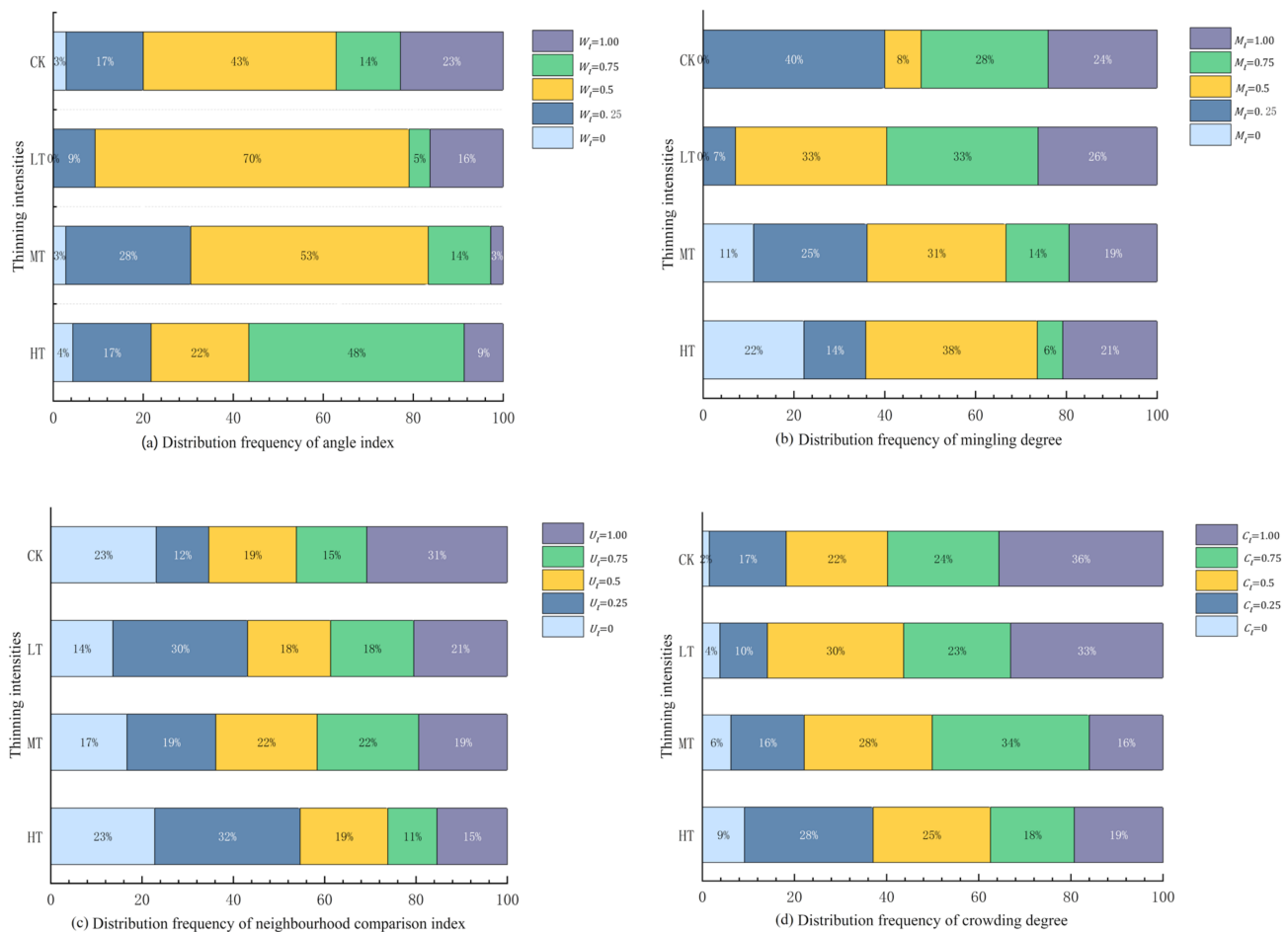
Figure 4. Distribution frequency of spatial structure index under different treatments. Pictures (a–d) represent angel index, mingling degree, neighbourhood comparison index and crowding degree, respectively.
