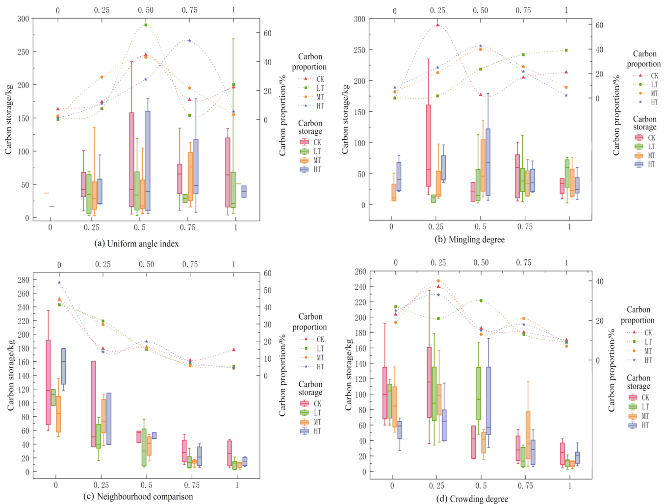
Figure 6. The carbon proportion of spatial structure index under different treatments. Pictures (a–d) represent uniform angle index, mingling degree, neighbourhood comparison and crowding degree, respectively.
