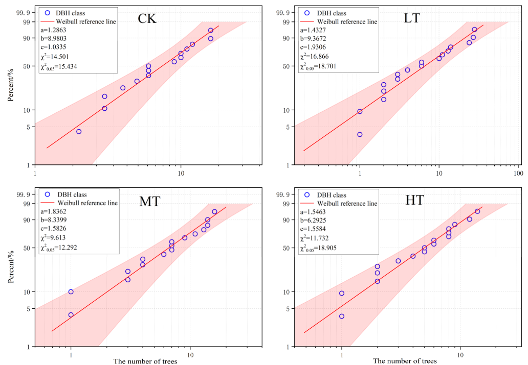
Figure 2. DBH frequency of Weibull distribution under different treatments. The results were subjected to \chi^2 test, and then the fitting results were analysed.
