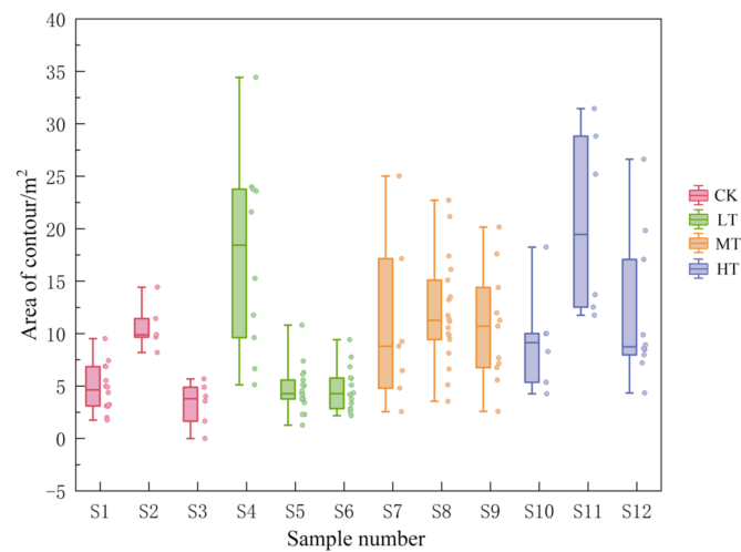
Figure 3. The effect of thinning on A -index under different treatments. The CK treatment included plots S1~S3, the LT treatment included plots S4~S6, the MT treatment included plots S7~S9, and the HT treatment included plots S10~S12.
