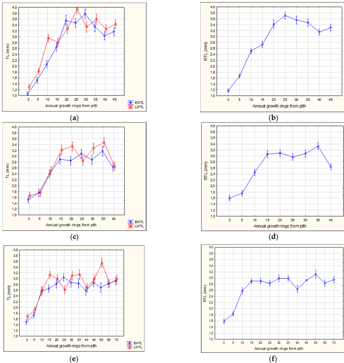
Figure 1. Radial trends of the P. menziesii tracheid length (EWTL—earlywood, LWTL—latewood, and RTL—annual ring) for all annual growth rings selected in wood from each site. (a,b) Veliki Grđevac; (c,d) Poreč; (e,f) Varaždin. The vertical bars represent 0.95 confidence intervals.
