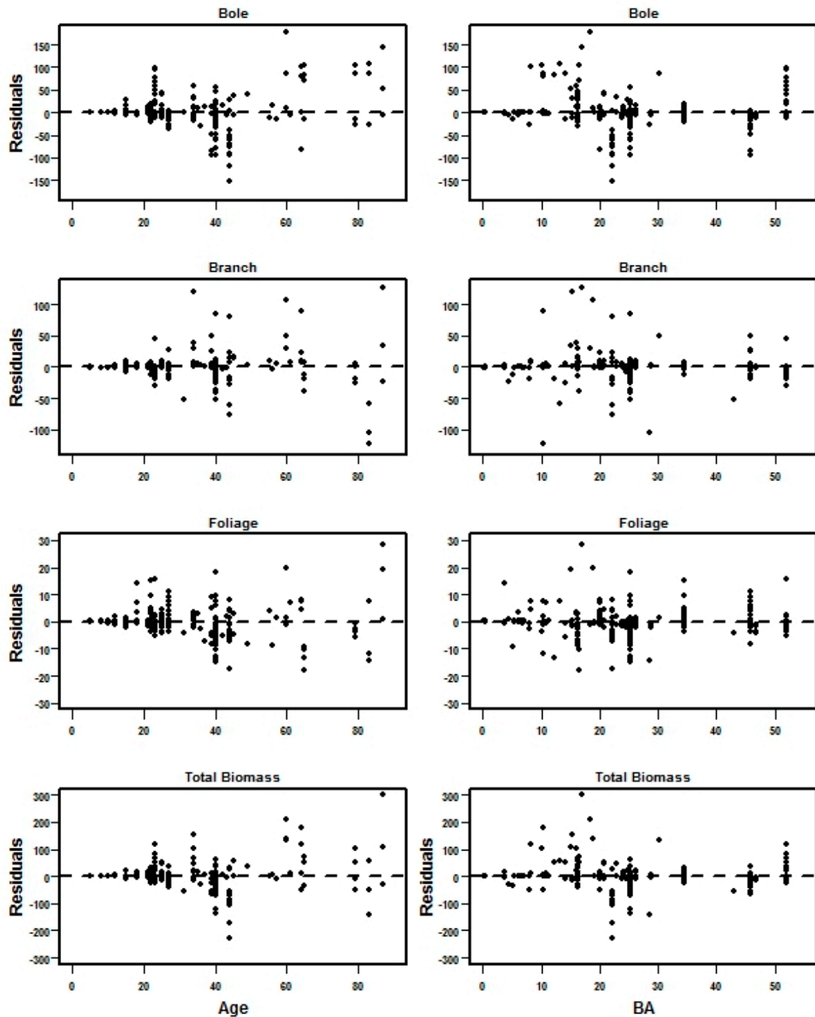
Figure S1: Pearson residual plots against age (left panel) and Basal Area (BA, right panel) for each biomass component in the model system VI fitted using NSUR method. There were not any obvious trends in the plots of biomass residuals against Age or BA.
