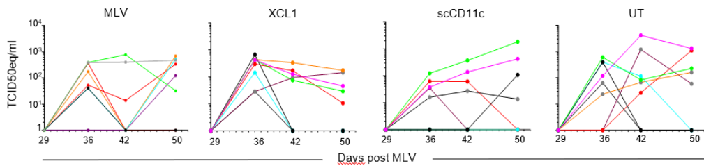
Supplementary Figure 1. Detection of MLV FL13b RNA in sera. The sera of the 4 DNA+MLV groups, collected on D29, 36, 42 and 50, were assayed for detection of MLV FL13b RNA using TaqMan qRT-PCR. TCID50eq/ml were calculated. The extrapolated TCID50eq/ml curves are shown for each pig represented by a distinct color.
