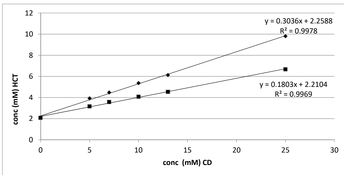
Figure S1. Phase solubility studies of HCT with SBEβCD (◆) and with HPβCD (■).
