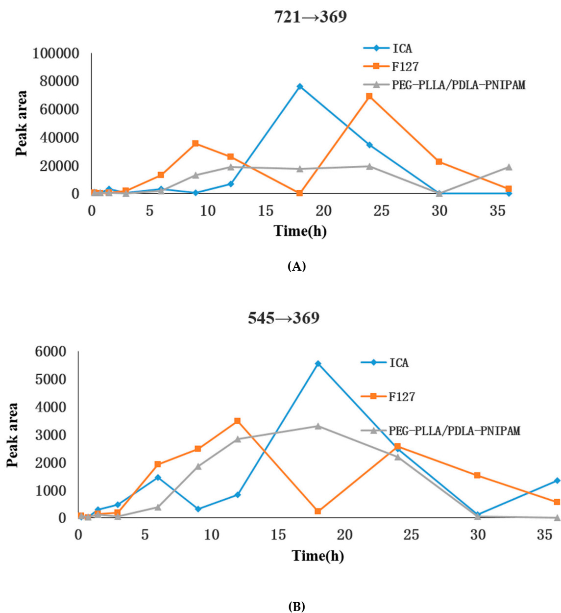
Figure S1. ICA in vivo metabolite product line chart. (A) 721→369; (B) 545→369.
