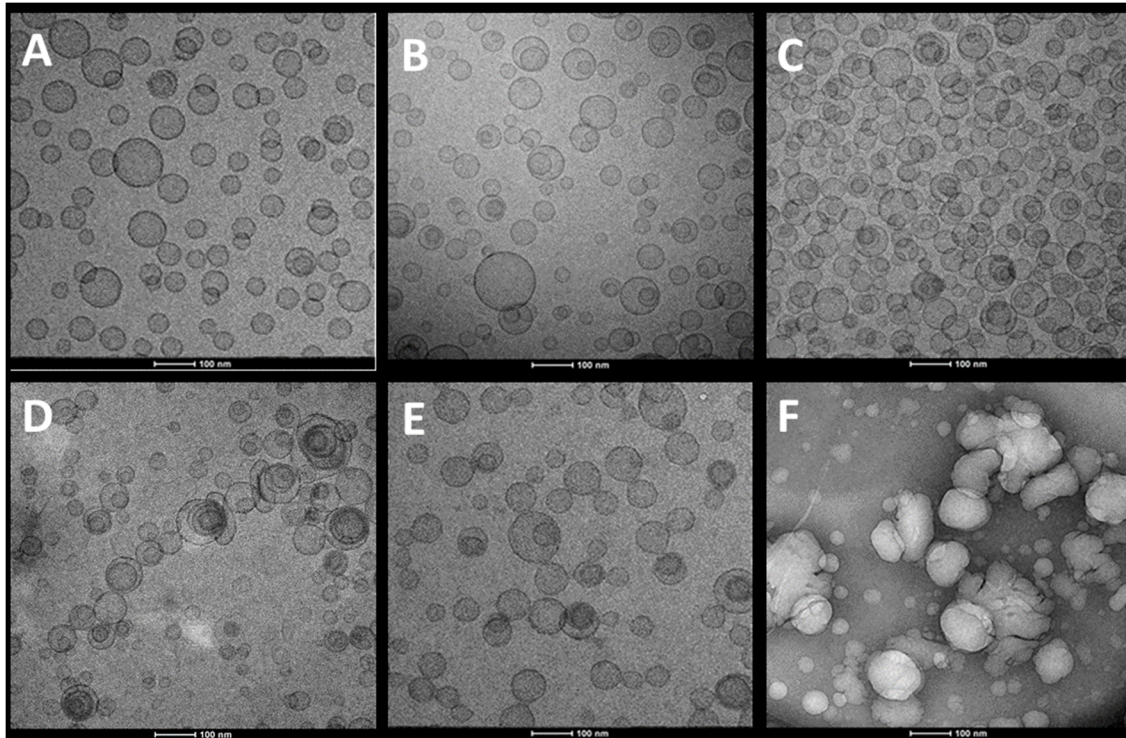
Figure 2. Representative cryo-TEM images of liposomes (A), glycerosomes (B,C), gluglycerosomes (D), gel-gluglycerosomes (E), and hyal-gluglycerosomes (F), loading H. scruglii extract.
