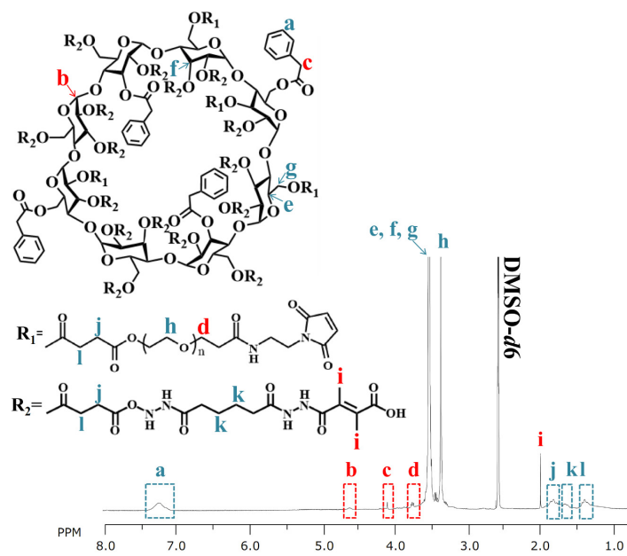
Figure S1. ^1\text{H-NMR} peaks of \gamma\text{CDP-(DMA/PEG)} .
