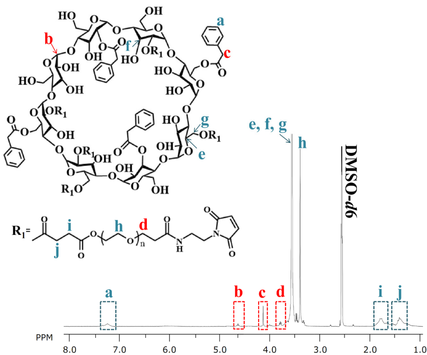
Figure S2. ^1\text{H-NMR} peaks of \gamma\text{CDP-(PEG)} .
