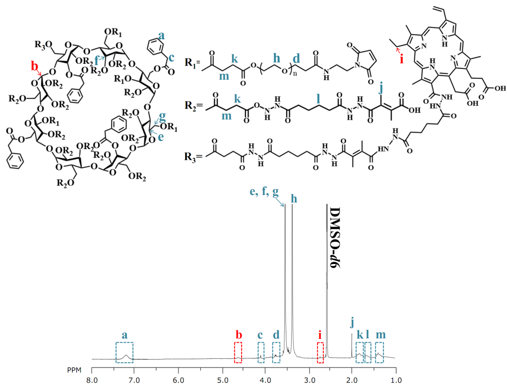
Figure S3. ^1\text{H-NMR} peaks of Ce6 dye-tagged \gamma CDP-(DMA/PEG).
