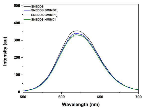
Figure S1. Fluorescence spectra of the SNEDDS diluted 1:100 in water.
