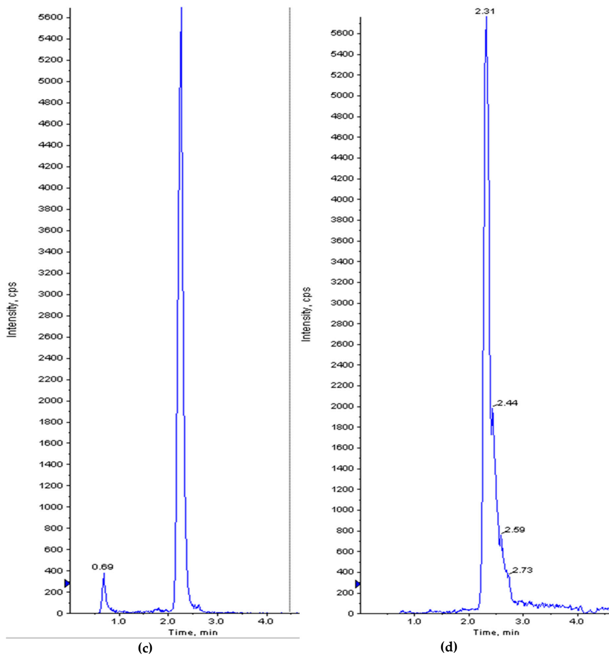
Figure S2. Chromatograms of LC-MS/MS of SNEDDS (a), SNEDDS:BMIMBF 4 (b), SNEDDS:BMIMPF 6 (c) and SNEDDS:HMIMCl (d), after 4 weeks.
