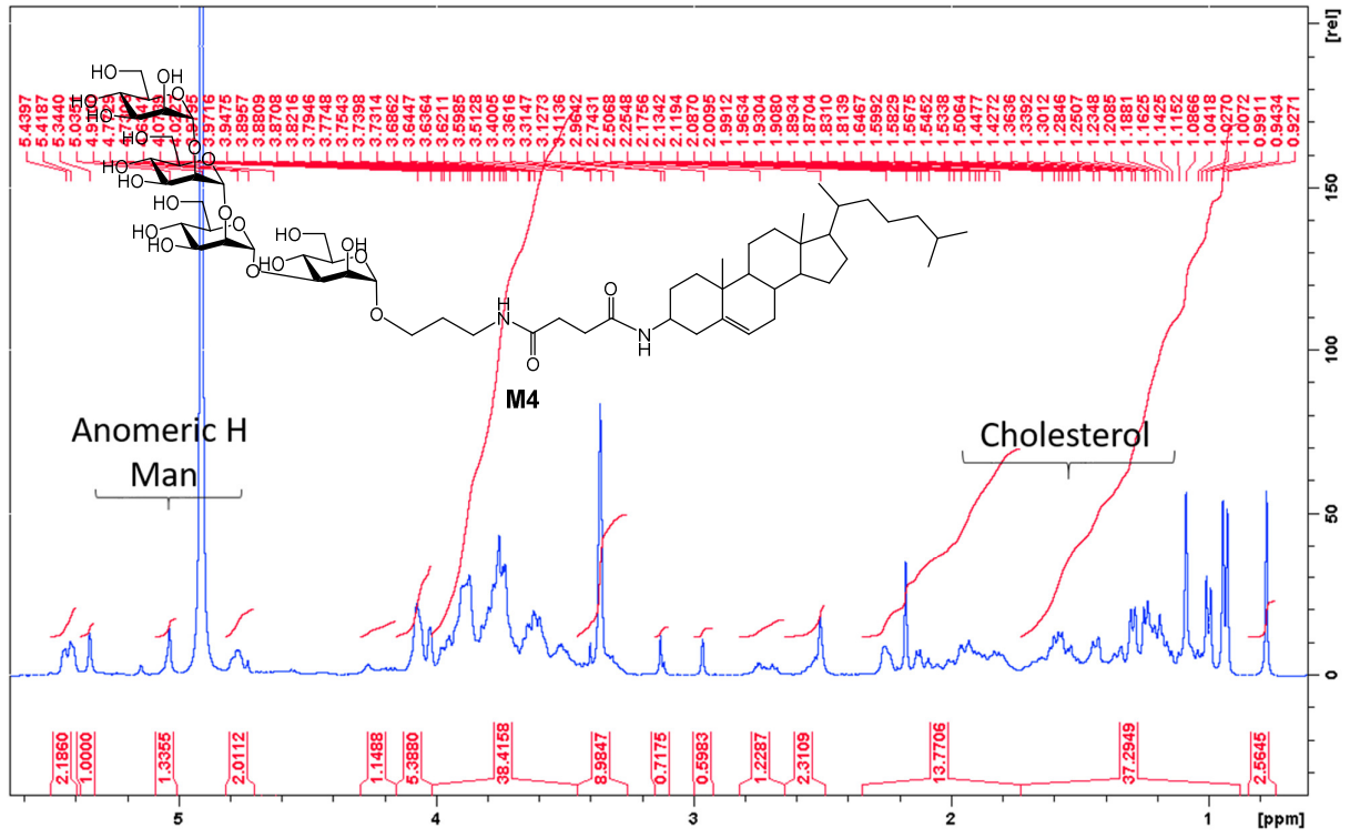
Figure S4. 1 H NMR (400 MHz, MeOD) of conjugate M4.
