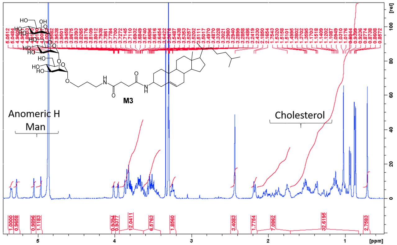
Figure S3. 1 H NMR (400 MHz, MeOD) of conjugate M3.
