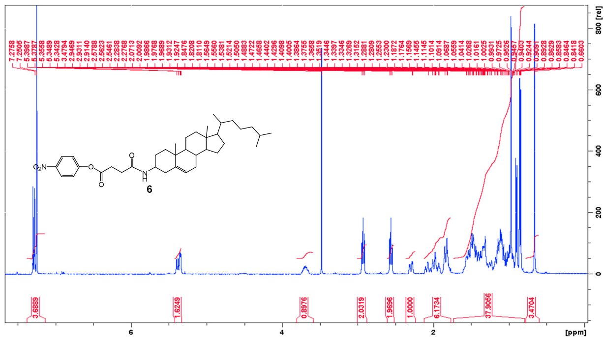
Figure S1. 1 H NMR (400 MHz, CDCl 3 ) of the cholesterol derivative 6.
