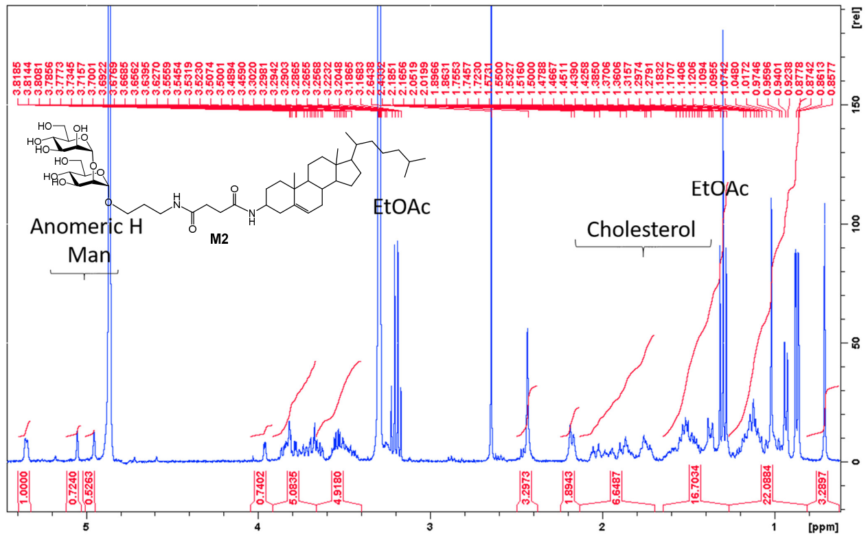
Figure S2. 1 H NMR (400 MHz, MeOD) of conjugate M2.
