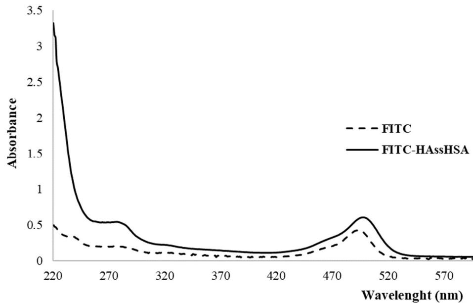
Figure S1. UV-vis spectra of FITC ( 4 \mu\text{g mL}^{-1} ) and FITC-HAssHSA ( 0.4 \text{ mg mL}^{-1} ) dissolved in carbonate buffer (100 mM, pH 9.2).
