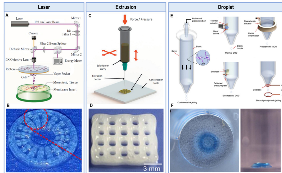
Figure 1. 3D bioprinting technologies and printed constructs (adapted with permission from [11,15,43–46]).
