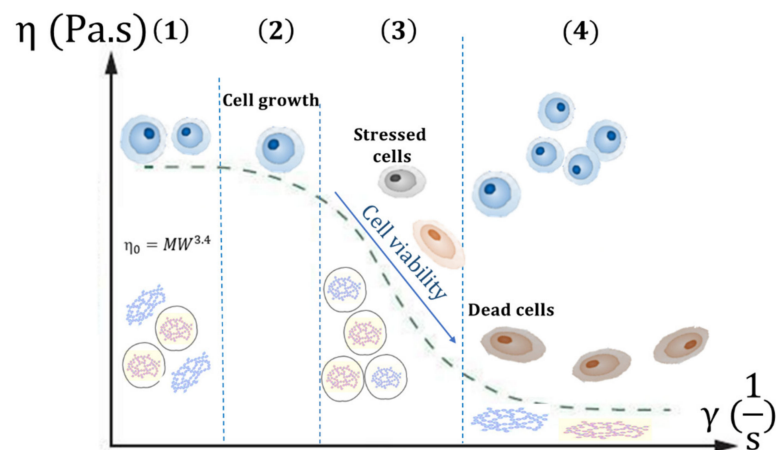
Figure 3. Shear–viscosity profile and respective cell behavior: (1) Zero shear viscosity; (2); Polydispersity –increases with broader MW; (3) Shear-thinning—Linear region—ideal conditions for extrusion; (4) Infinite shear-rate [133–135].
