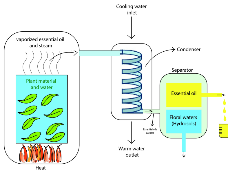
Figure 10. Essential oils processing units.
