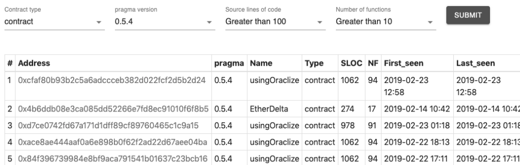
Figure 5. Smart Corpus’s user interface.
