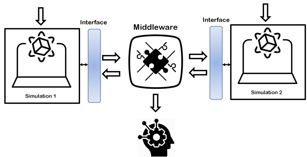
Figure 6. Middleware implementation.
