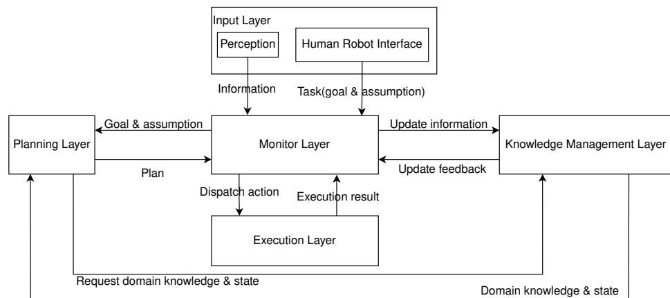
Figure 1. Framework overview.
